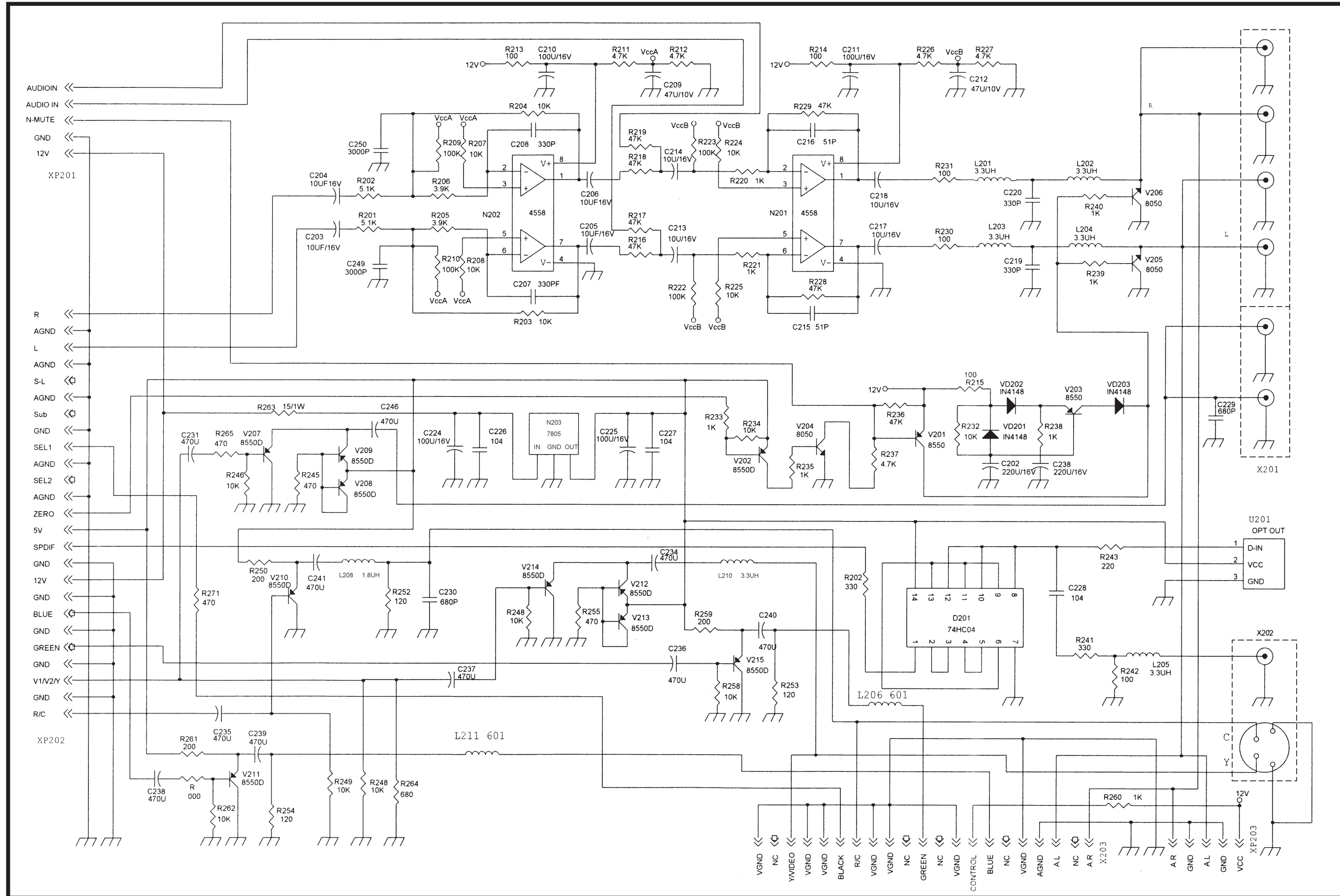
SCART-868-312P OUTPUT CIRCUIT
