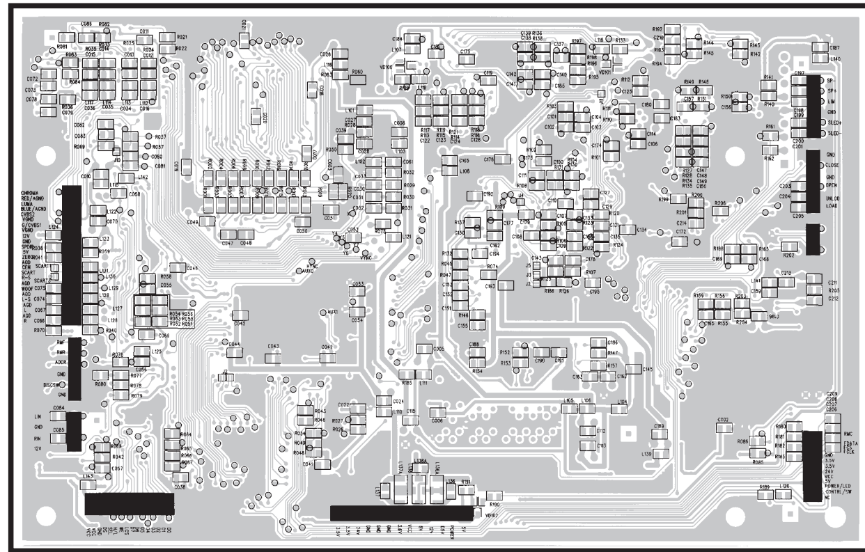
DSM6012BM MAIN BOARD
